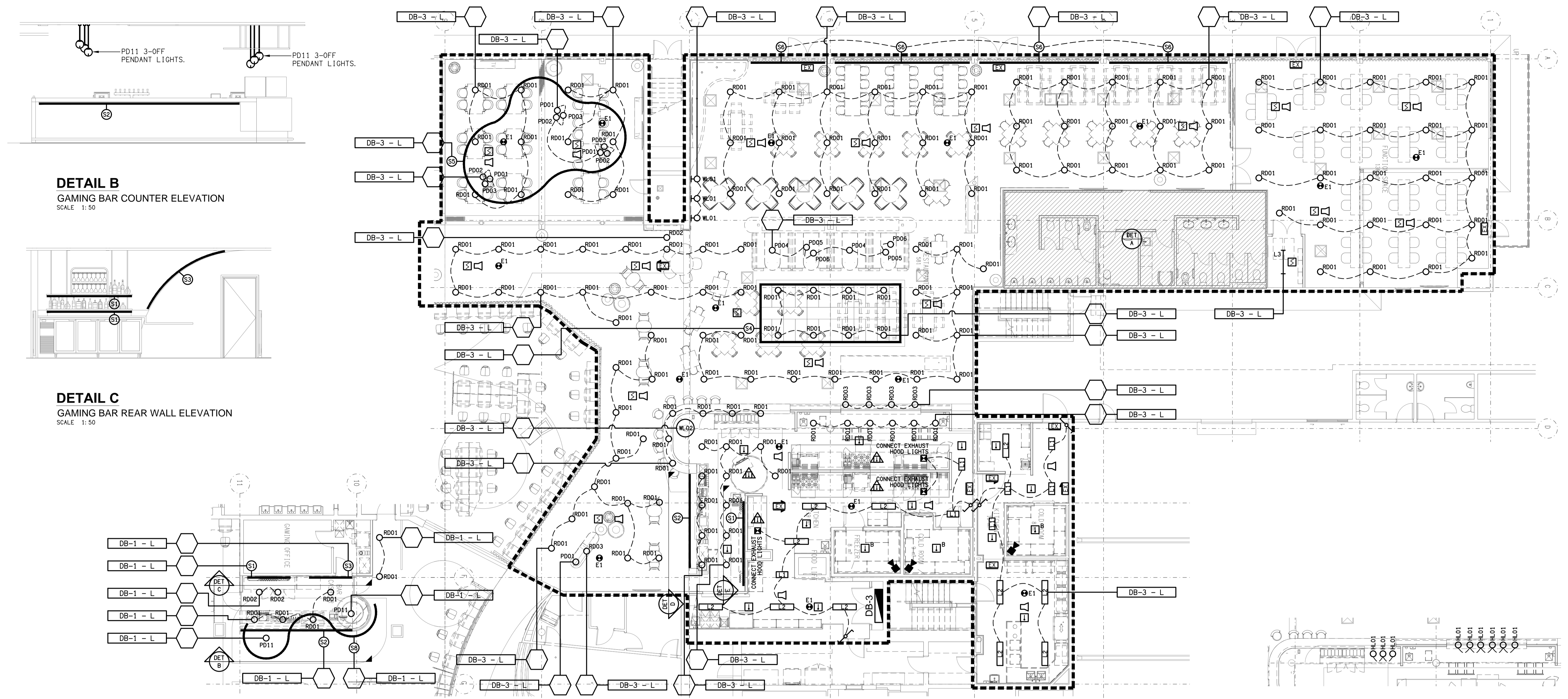
REFLECTED CEILING PLAN REFURBISHMENT SCALE 1:100
