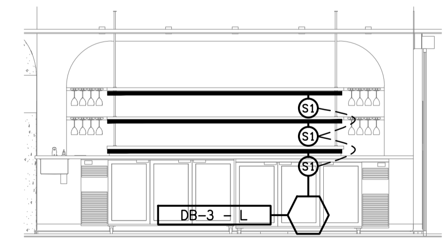
DETAIL E BAR REAR WALL SHELVING ELEVATION SCALE 1:50
