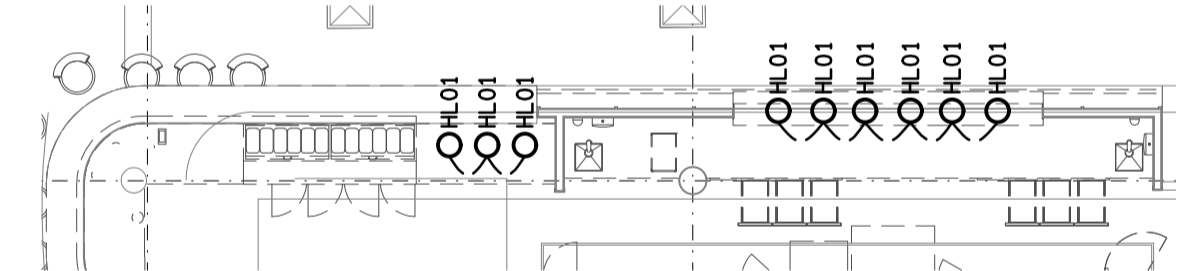
DETAIL F SERVERY HEAT LAMP PLAN SCALE 1:100
