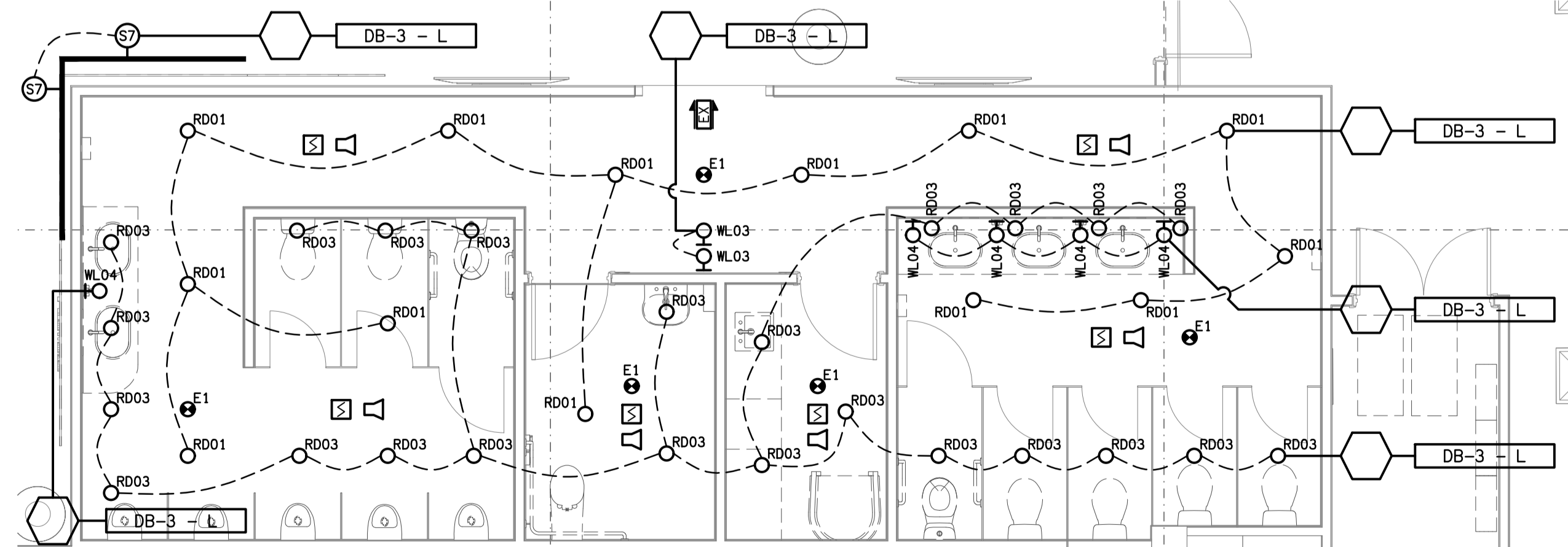
DETAIL A AMENITIES REFLECTED CEILING PLAN SCALE 1:50
