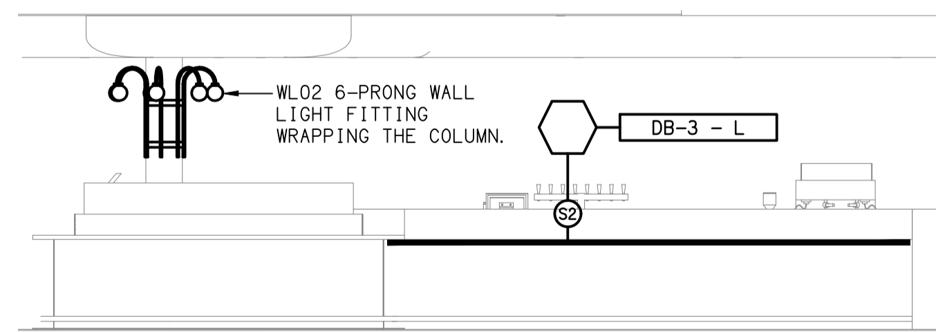
DETAIL D BAR COUNTER ELEVATION SCALE 1:50
