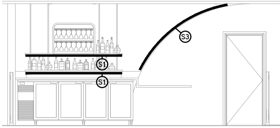
DETAIL C GAMING BAR REAR WALL ELEVATION SCALE 1:50
